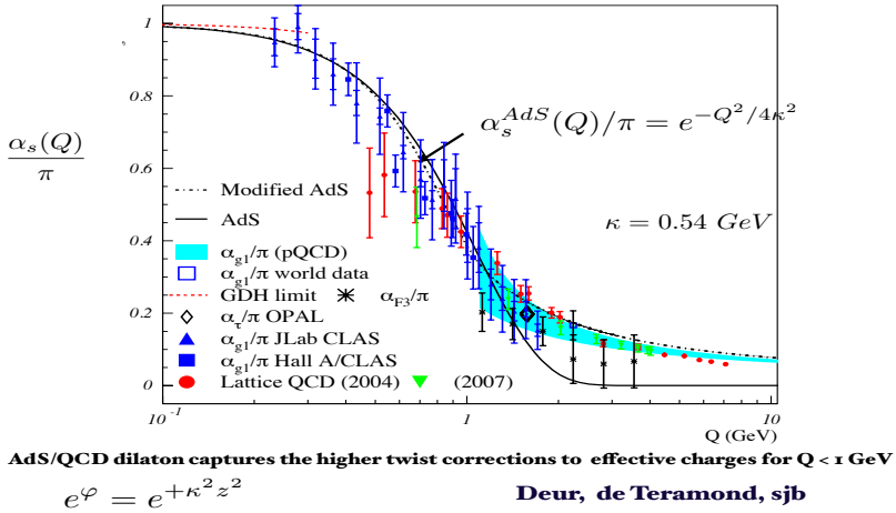
Fig.4.1: (A). Prediction from LF Holography for the QCD running coupling \alpha_{g_1}^s(Q^2) . The magnitude and derivative of the perturbative and nonperturbative coupling are matched at the scale Q_0 . This matching connects the perturbative scale \Lambda_{\overline{MS}} to the nonperturbative scale \kappa which underlies the hadron mass scale. (B). Comparison of the predicted nonperturbative coupling with measurements of the effective charge \alpha_{g_1}^s(Q^2) defined from the Bjorken sum rule. See Ref. [28].
