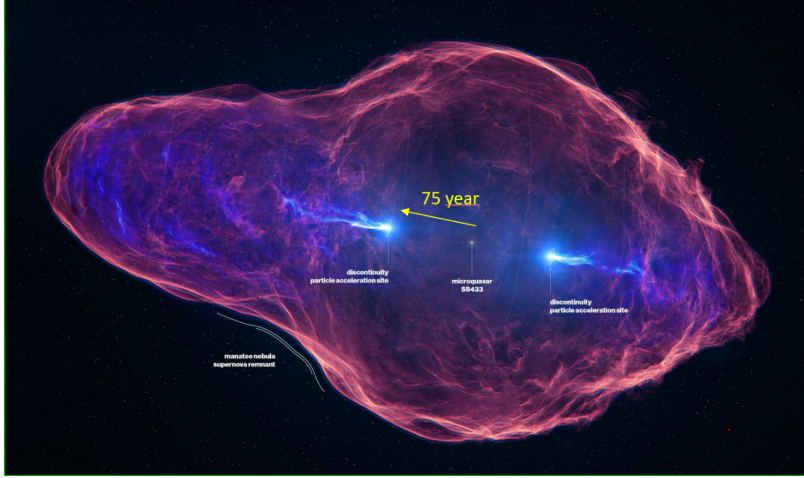
Fig. 5.1: A simplified description of the separated TeV beam observed by Hess, HAWC and LHAASO. The resurgence of the collimated gamma beam at 75y \cdot c is very puzzling.
