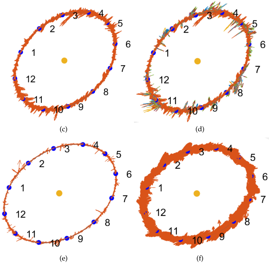
Fig. 6.2: Difference vectors \overline{DV} in relation to the Earth's orbit: Proton Flux >1 MeV (a), Proton Flux >1 MeV [orange], >10 MeV [green], >60 MeV [blue] (b), Dst (c), Dst [orange] and all Proton Fluxes (d), SW Plasma Temperature (e), F10.7 (f).
