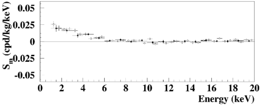
Fig. 1.4: Comparison between the modulation amplitudes, S_m , for the whole data set (open circles): DAMA/NaI, DAMA/LIBRA-phase1 and DAMA/LIBRA-phase2 (total exposure 2.86 ton \times yr) and for the data set (black circles) of the last three published years of DAMA/LIBRA-phase2 (in which there was continuity between one year and the next) analyzed considering the same background, see text. The modulation amplitudes of the two data sets are compatible, implying that any effect of long-term time-varying background or odd low-energy rate increasing with time is negligible in DAMA/LIBRA, thanks to the radiopurity and long-time underground of the ULB DAMA/LIBRA NaI(Tl). Thus, the original DAMA analyses can be safely adopted.
