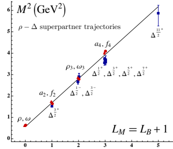
Fig. 4.3: Comparison of the \rho/\omega meson Regge trajectory with the J = 3/2 \Delta baryon trajectory. Superconformal algebra predicts the degeneracy of the meson and baryon trajectories if one identifies a meson with internal orbital angular momentum L_M with its superpartner baryon with L_M = L_B + 1 . See Refs. [7, 8].
