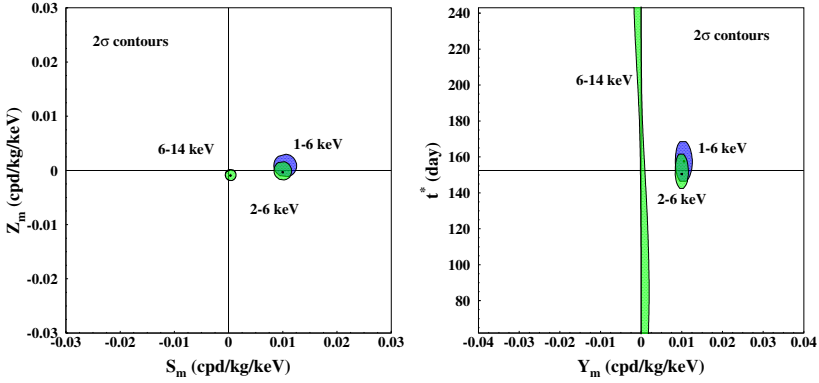
Fig. 1.3: 2\sigma contours in the plane (S_m, Z_m) (left) and in the plane (Y_m, t^*) (right) for: i) DAMA/NaI, DAMA/LIBRA-phase1 and DAMA/LIBRA-phase2 in the (2 – 6) keV and (6 – 14) keV energy intervals (light areas, green on-line); ii) only DAMA/LIBRA-phase2 in the (1 – 6) keV energy interval (dark areas, blue on-line). The contours have been obtained by the maximum likelihood method. A modulation amplitude is present in the lower energy intervals and the phase agrees with that expected for DM induced signals.
