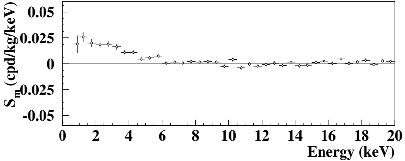
Fig. 1.2: Modulation amplitudes, S_m , as function of the energy for the whole data sets: DAMA/NaI, DAMA/LIBRA-phase1 and DAMA/LIBRA-phase2 (total exposure 2.86 \text{ ton} \times \text{yr} ) above 2 keV; in the bin (1 – 2) keV only the DAMA/LIBRA-phase2 exposure ( 1.53 \text{ ton} \times \text{yr} ) is available and used, while the first lowest energy point has been obtained by a cautious re-analysis with specific dedicated efficiency analysis there. A clear modulation is present in the lowest energy region, while S_m values compatible with zero are present just above.
