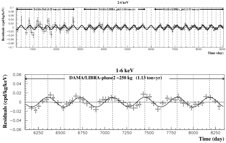
Fig. 1.1: Top : Experimental residual rate of the single-hit scintillation events measured by DAMA/NaI, DAMA/LIBRA–phase1 and DAMA/LIBRA–phase2 (total exposure 2.86 \text{ ton} \times \text{yr} ) in the (2 – 6) keV energy intervals as a function of the time. The superimposed curve is the cosinusoidal functional forms A \cos \omega(t - t_0) with a period T = \frac{2\pi}{\omega} = 1 \text{ yr} , a phase t_0 = 152.5 \text{ day} (June 2 nd ) and modulation amplitude, A , equal to the central value obtained by best fit. Vertical dashed lines indicate the expected maximum rate, while the dotted lines represent the expected minimum rate. Bottom : Experimental residual rate of single-hit scintillation events measured by DAMA/LIBRA–phase2, which operates with a lower software energy threshold, in the (1 – 6) keV energy range, shown as a function of time.
