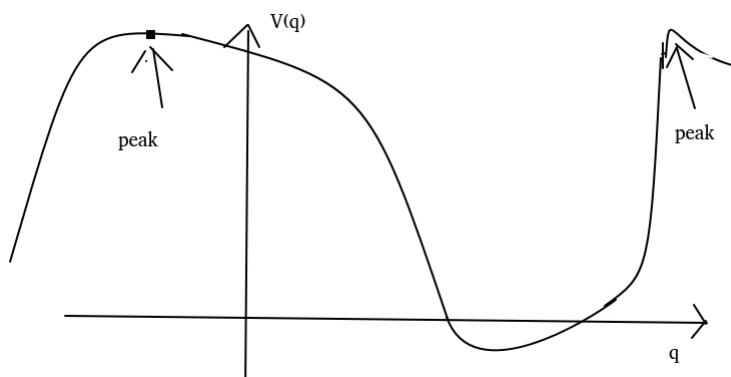
Fig. 14.2: Inflaton potential with two peaks
