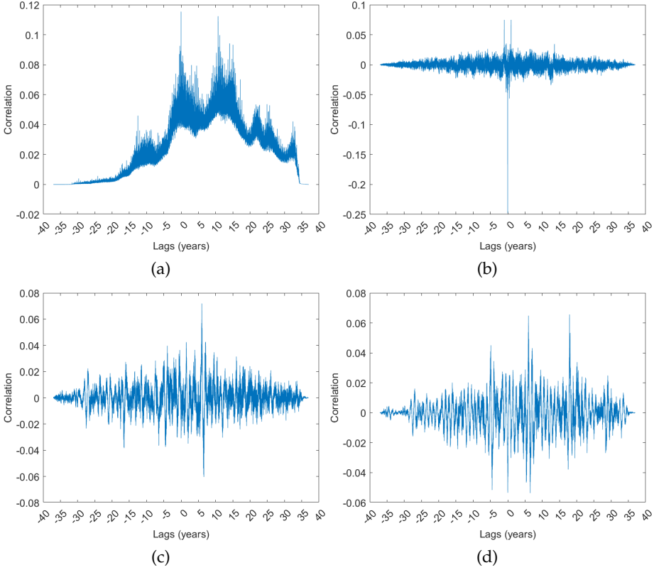
Fig. 6.4: Cross-correlation functions: \overline{DV}_{E_y} and \overline{DV}_{\text{Proton Flux} > 60 \text{ MeV}} (a), \overline{DV}_{A, \text{Flow Pressure}} and \overline{DV}_{A, \text{Dst}} (b), \overline{DV}_{A, \text{SW Proton Density}} and \overline{DV}_{A, \text{F10.7}} (c), \overline{DV}_{A, \text{Plasma Beta}} and \overline{DV}_{A, \text{F10.7}} (d).
