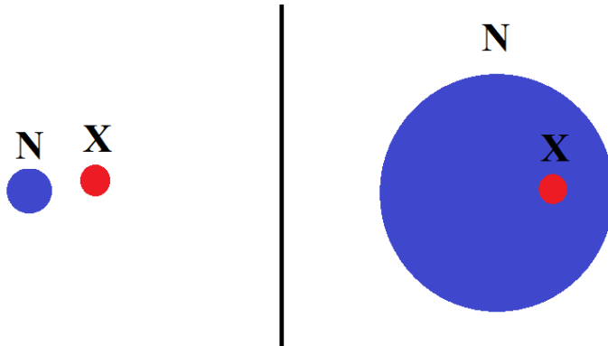
Fig. 2.1: Bohr-like (left) and Thomson-like (right) dark atoms
