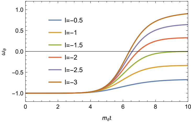
Fig. 9.2: The plot of the equation of state parameter for the scalar field. We see that scalar field could behave differently depending on the value of l and in particular, if l = -1.5 then scalar field behaves like non-relativistic matter.
