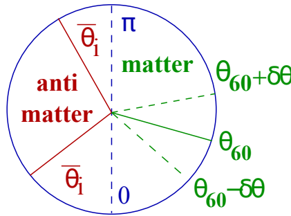
Fig. 7.1: Phase fluctuations at inflationary stage can cross \pi . It leads to formation of closed domain walls. If the ALP field is unstable relative to decays to quarks and leptons with baryon and lepton number nonconservation, as it is the case in the model of spontaneous baryosynthesis [28], crossing \pi and 0 , results in formation of antibaryon domains in baryon asymmetric Universe [1]
