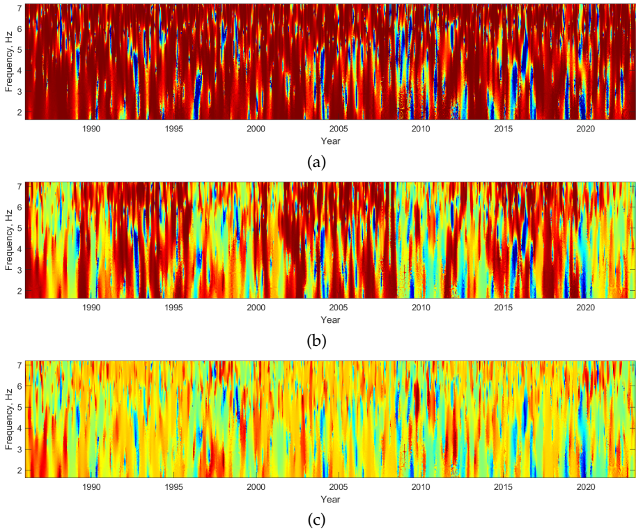
Fig. 6.5: Wavelet semblance for SSN and F10.7: WS(SSN, F10.7) (a), averaged WS(SSN, F10.7) and WS(SSN, |\overline{DV}|_{F10.7}) , WS(SSN, |\overline{DV}|_{s, F10.7}) (b), averaged WS(SSN, F10.7) and WS(SSN, |\overline{DV}|_{F10.7}) , WS(SSN, \text{sign} \cdot |\overline{DV}|_{F10.7}) (c).
