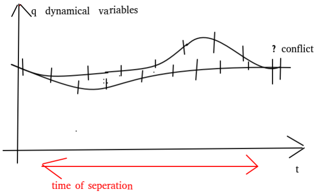
Fig. 14.5: Clocks beat differently on paths
