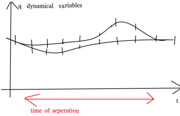
Fig. 14.4: A "clock" beating disconnected
