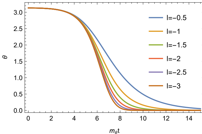
Fig. 9.1: The plot of the solution of (9.36) for different values of l , where the interesting observation is the impact of l changing slowly for l < -2 .
