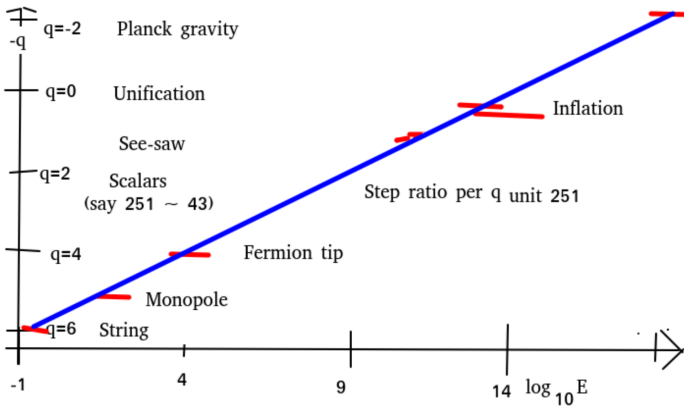
Figure 3: This figure taken from [2] has the logarithm in basis 10 of the energy scales on the abscissa, and the integer q = 4 - n , where n is essentially the power of 1/a relevant for the scale. Remark that we have -q as the variable pointing upwards. The names we have given to the scales are attached.
