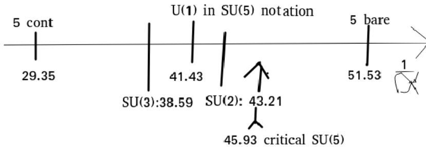
Figure About Critical Coupling
