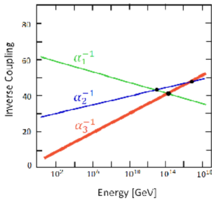
Figure 4: This is the usual graph representing the three Standard Model inverse fine structure constants with the \alpha_1^{-1} being in the notation suitable for SU(5) , meaning it is 3/5 times the natural normalization, \alpha_{1\ SU(5)}^{-1} = 3/5 * \alpha_{1\ SM}^{-1} = 3/5 * \alpha_{EM}^{-1} \cos^2 \Theta_W . The vertical thin line at the energy scale \mu_U = 5 * 10^{13} GeV points out “our unified scale”, which is as can be seen not really unifying the couplings, but rather is the scale where the ratio of the two independent differences, \alpha_2^{-1} - \alpha_{1\ SU(5)}^{-1} and \alpha_{1\ SU(5)}^{-1} - \alpha_3^{-1} have just the ratio 2/3 as our model predicts at the “our unification scale”. One may note, that this “our unified scale” is actually very close to, where the three inverse couplings are nearest to each other, and in that sense an “approximate” unification scale.
